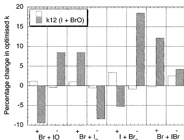
Figure 5. Sensitivity test 2. The sensitivity of the optimized values of k_1 and k_{12} to the rate coefficient of selected secondary reactions included in the reaction model.
