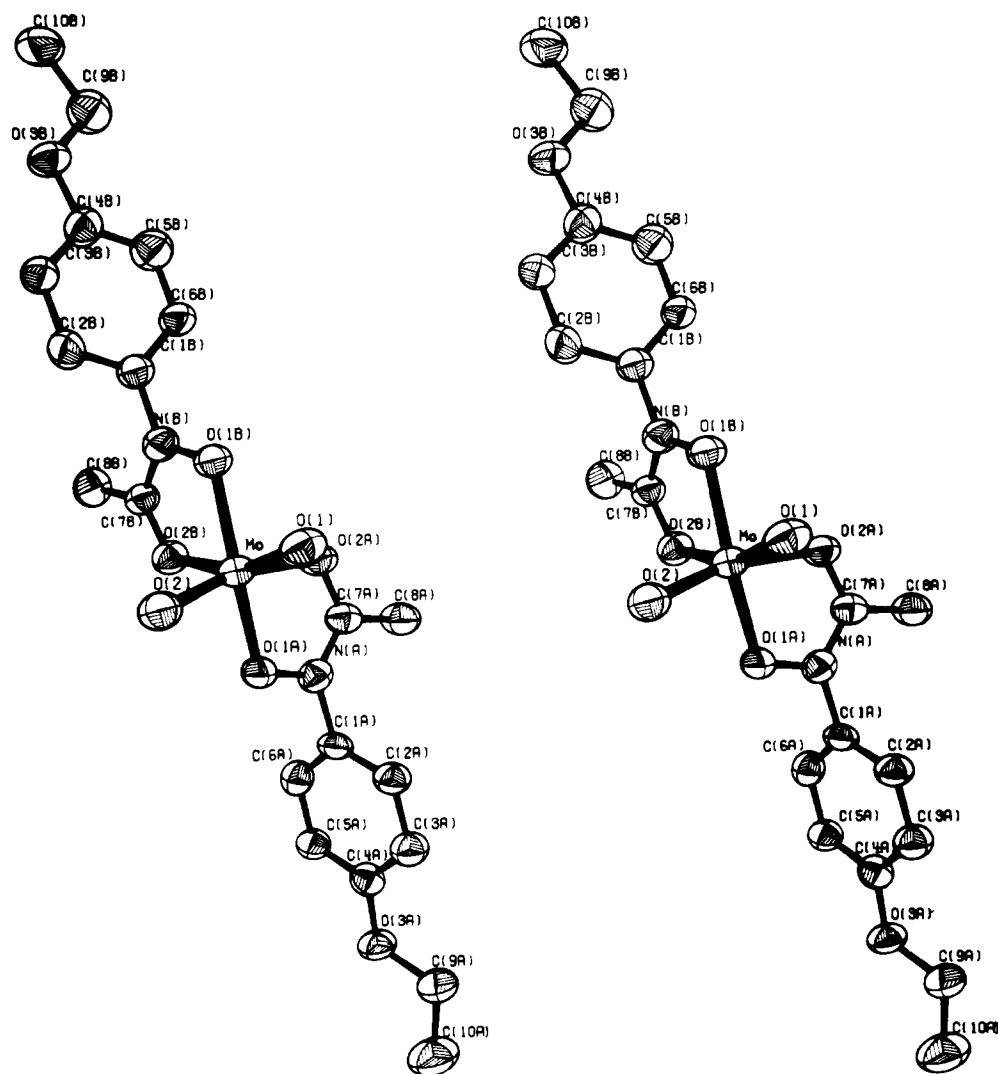
Figure 3. Stereoview of the \text{MoO}_2\text{L}_2 molecule, the complex of the phenacetin metabolite.
