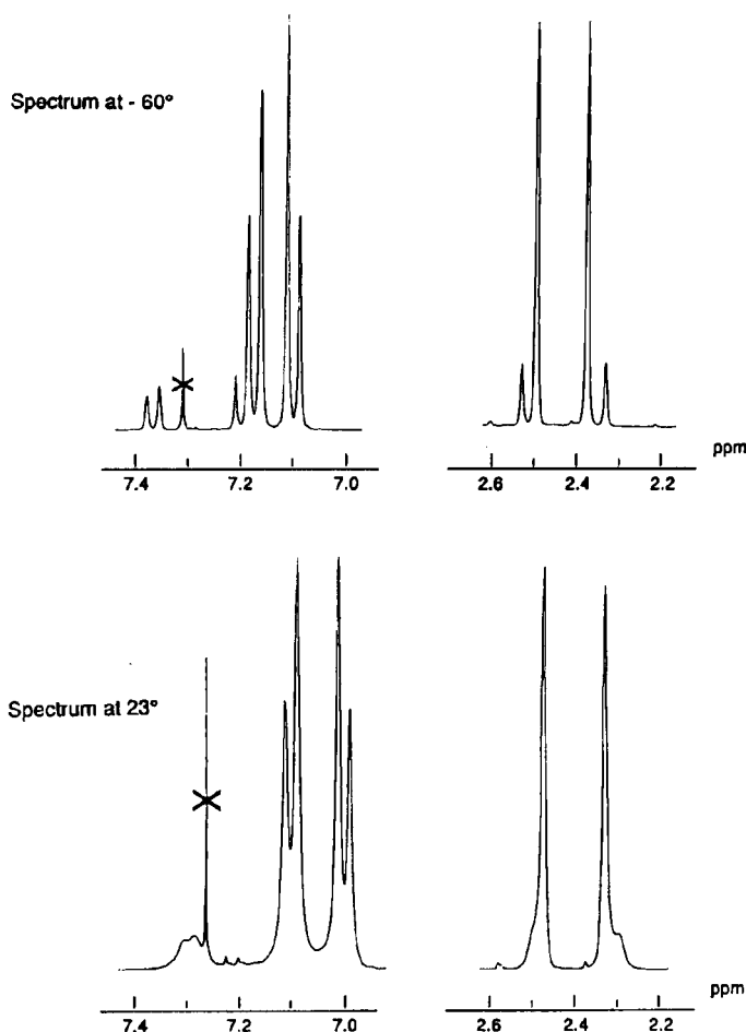
Figure 1. Low and Room Temperature nmr Spectra of Compound 3.
