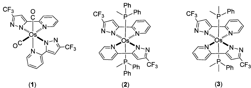
Scheme 2. Structural Drawing of Osmium(II) Complexes with the Bidentate fpz Chelate
