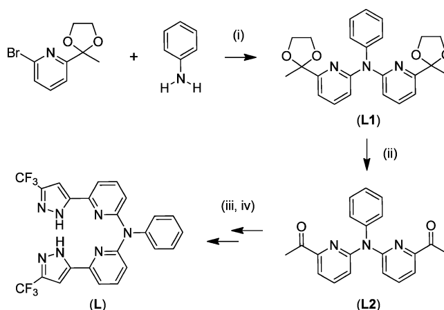
Scheme 1. Synthetic Procedures to the Tetradentate Chelate L a
