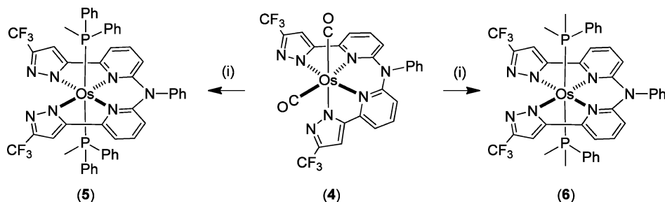
Scheme 3. Transformation of Osmium(II) Complexes with the Tetradentate Chelate L a
