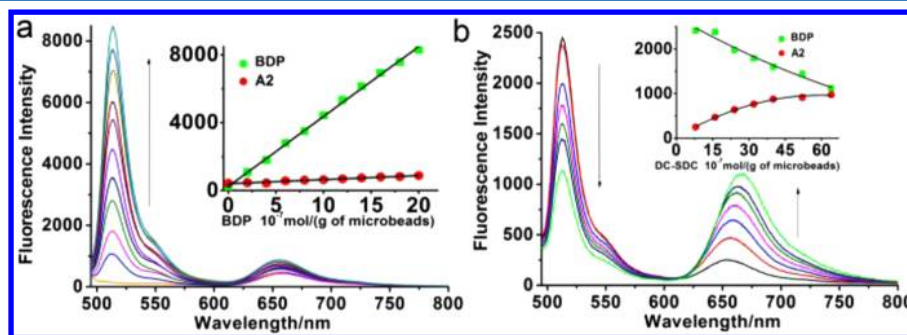
Figure 4. Fluorescence spectra changes of microspheres (in water, \lambda_{\text{ex}} = 480 nm) labeled by BDP ( \lambda_{\text{em}} = 512 nm) and A2 ( \lambda_{\text{em}} = 656 nm). (a) Fluorescence spectra change vs doping amount of BDP , inset: intensity of emission maxima vs amount of BDP . (b) Fluorescence spectra change vs doping amount of A2 , inset: intensity of emission maxima vs amount of A2 ; unit 10^{-7} mol/(g of microspheres).
