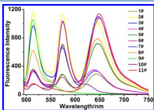
Figure 3. Fluorescence spectra of triple labeled microspheres in water ( \lambda_{\text{ex}} = 480 nm, \lambda_{\text{em}} = 490\text{--}750 nm, slit 5 nm, 5 nm).
