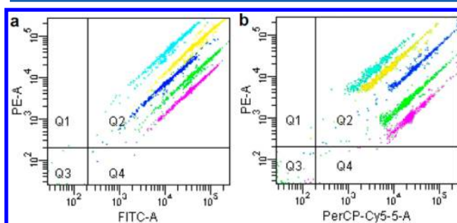
Figure 6. Flow cytometric analysis of a mixture sample of five microspheres: (a) co-doping by BDP and BDP-A1, FITC-A is the name for green channel: 530 \pm 30 \text{ nm} ; PE-A is the name for red channel: 585 \pm 42 \text{ nm} ; (b) co-doping by BDP-A1 and BDP-A2, PE-A is the name for red channel: 585 \pm 42 \text{ nm} ; PerCP-Cy5.5-A is the name for NIR channel: 670LP.
