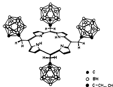
Figure 1. The proposed \alpha,\alpha,\alpha,\beta atropisomer of \text{H}_2[\text{P}(\text{CH}_2\text{C}_2\text{B}_{10}\text{H}_{10}\text{Me})_4] ( 11 ) and \text{H}_2[\text{P}(\text{CH}_2\text{C}_2\text{B}_{10}\text{H}_{11})_4] ( 6 ).
