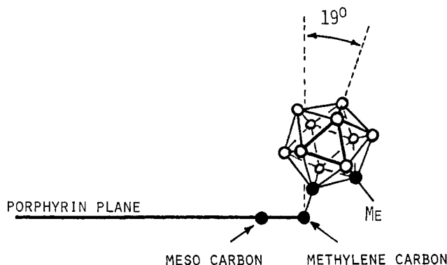
Figure 2. Depiction of preferred geometry of meso - \text{CH}_2\text{-C}_2\text{B}_{10}\text{H}_{11}\text{Me} moiety based on space-filling models.
