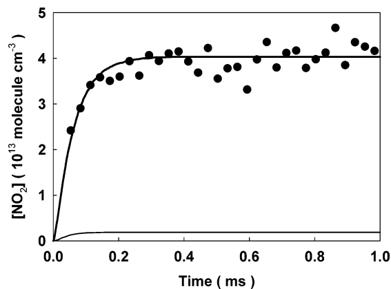
Figure 5. Temporal profile of NO 2 observed in an experiment at 213 K using the following reagent concentrations (molecule cm -3 ): O 2 , 4.0 \times 10^{18} ; N 2 , 4.7 \times 10^{17} ; Cl 2 , 1.9 \times 10^{16} ; NO, 1.6 \times 10^{15} . The solid circles are experimental results. The thick and thin curves are results of simulations using Y_{\text{NO}_2} = 0.18 and 0.00, respectively.
