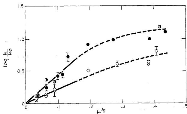
Figure 1.—Ionic strength effects in the reaction of \text{Ru}(\text{NH}_3)_6^{+2} with \text{Co}(\text{III}) complexes.
