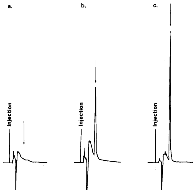
Figure 1 —HPLC traces of extracts of distilled water that had been standing in Brand C (sensitivity 0.05 a.u.s) (a), Brand B (0.02 a.u.s) (b), and Brand A (0.05 a.u.s) (c) syringes. The arrow marks retention time of 6.5 min.
