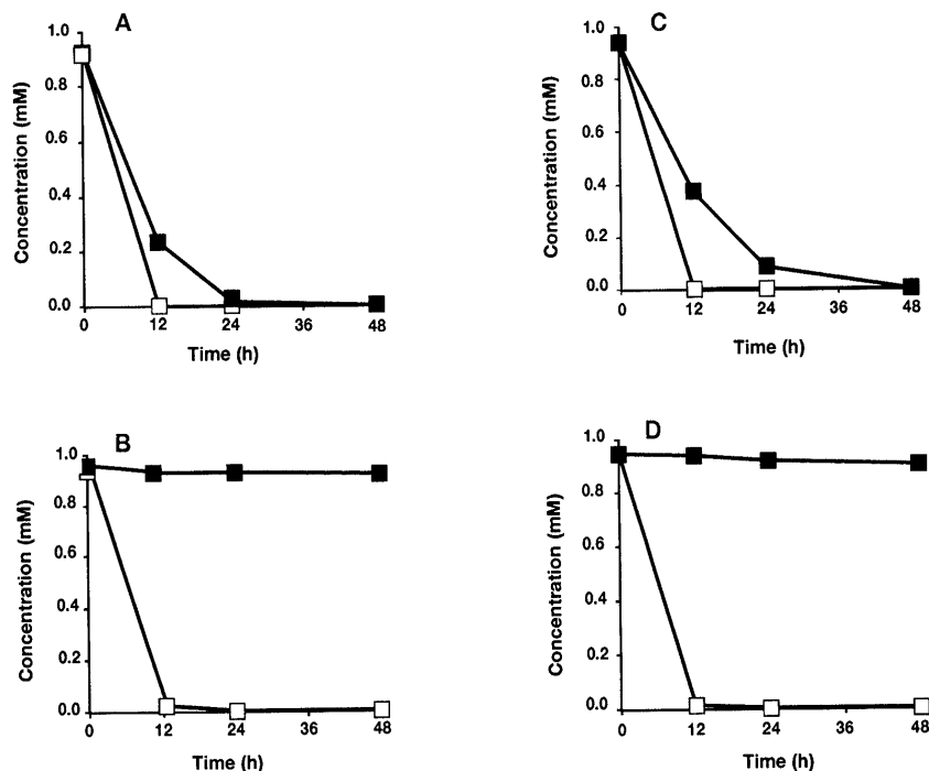
Fig. 1. Comparative Degradation Curves of Flavan-3-ols and Their Gallates by HIB (□) and RIB (■)
