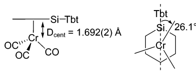
Figure 2. Distance ( D_{\text{cent}} ) between the silabenzene ring and the Cr center (left) and the projection of \text{Cr}(\text{CO})_3 onto the silabenzene ring plane (right).
