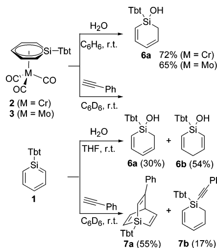
Scheme 2. Comparisons of Reactivities of Silabenzene Complexes ( 2 and 3 ) with Those of Silabenzene 1
