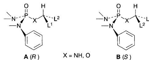
Fig. 1 Configurations of A and B (L 1 > L 2 )
