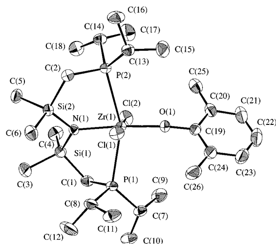
Figure 1. ORTEP drawing showing the molecular structure and numbering scheme for Zr(O-2,6-Me 2 C 6 H 3 )Cl 2 [N(SiMe 2 CH 2 PPr i 2 ) 2 ] ( 5 ). Ellipsoids are drawn at the 33% probability level.
