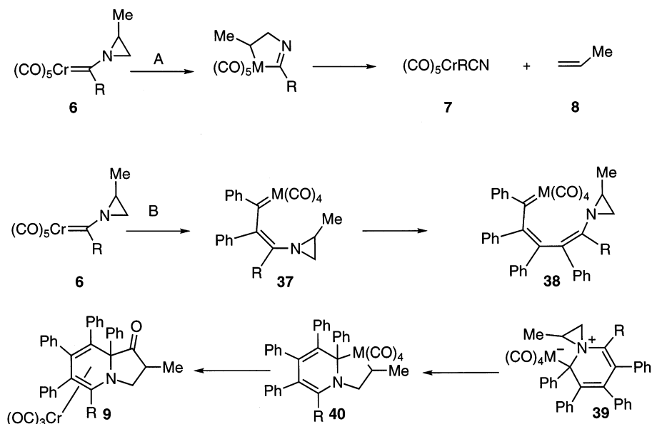
Scheme 5.
