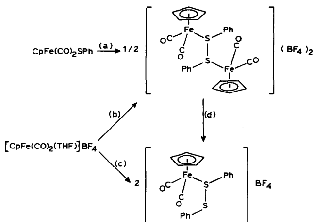
SCHEME 1. (a) \text{AgBF}_4 or \text{NOPF}_6 (yielding \text{PF}_6^- salt); (b) 0.5 equiv. \text{PhSSPh} , (c) 1.0 equiv. \text{PhSSPh} ; (d) \text{CH}_3\text{CN} ; [\text{CpFe(CO)}_2(\text{MeCN})]\text{BF}_4 is the second product.
