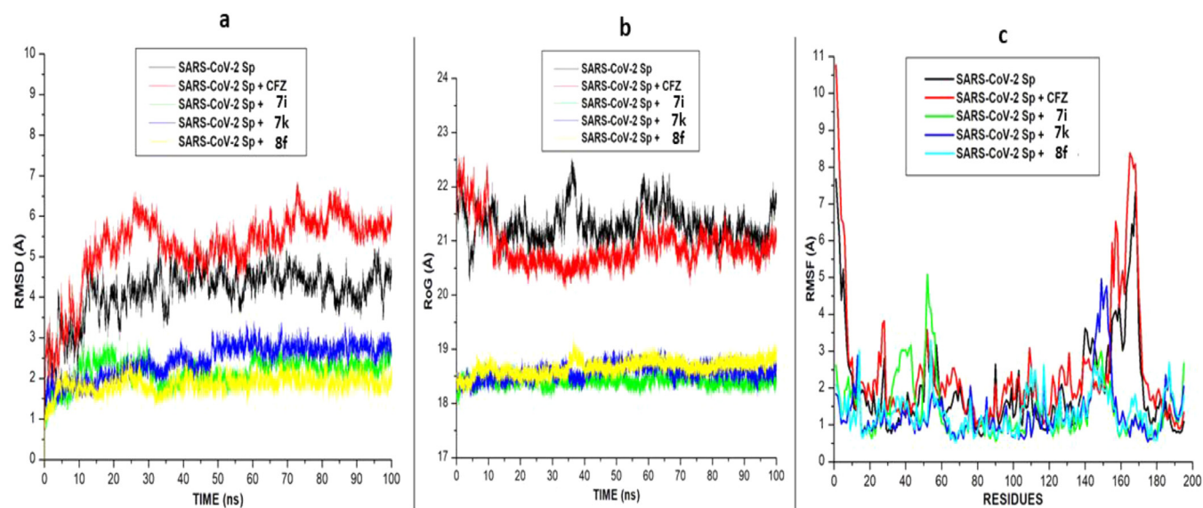
Fig. 4. Comparative (a). RMSD (b). RoG, and (c). RMSF plots of alpha C atoms of the SARS-CoV-2 S_{gp} systems calculated throughout 100 ns MD simulations.
