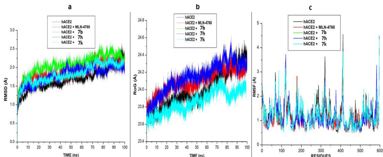
Fig. 5. (a) Comparative (a). RMSD (b). RoG, and (c). RMSF plots of alpha C atoms of the hACE-2 systems calculated throughout 100 ns MD simulations. (b): Comparative (a). RMSD (b). RoG, and (c). RMSF plots of alpha C atoms of the hACE-2 systems calculated throughout 100 ns MD simulations.
