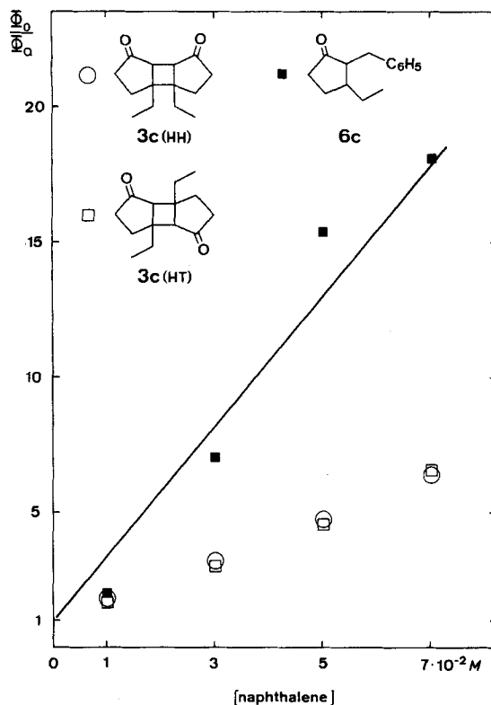
Fig. 2. Stern-Volmer Plots for Quenching of Photoproducts: 1c + Naphthalene 0.09M Degassed solution of 1c in toluene at > 3400 \text{ \AA} ; maximum conversion ca. 10%. Tentative structural assignment to 3c (HH) and 3c (HT) by analogy with relative VPC retention times of 3b (HH and anti-HT) and 3d (HH and HT)
