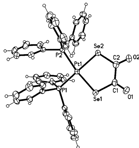
Figure 4. ORTEP plot of the molecular structure of [\text{Pt}(\eta^2\text{-Se}_2\text{C}_2\text{O}_2\text{-Se,Se}')(\text{PPh}_3)_2] ( 6 ) with 50% probability thermal ellipsoids.
