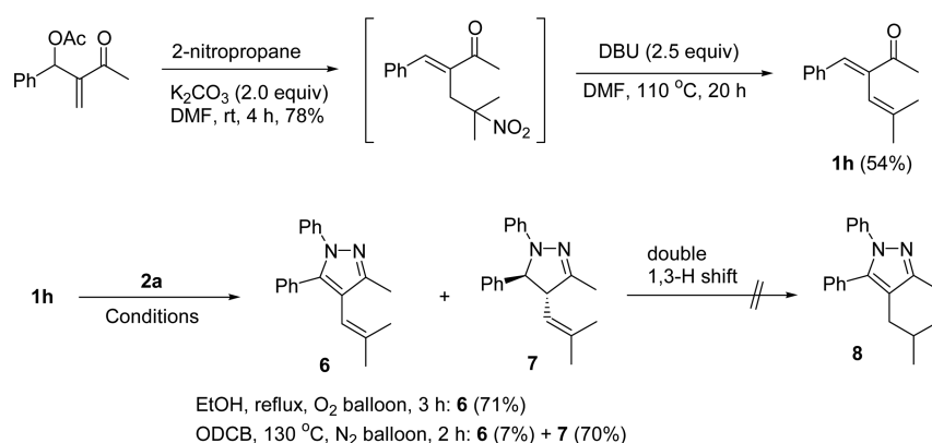
Scheme 4
