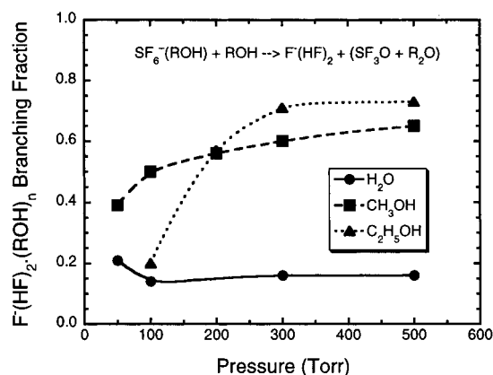
Figure 6. Pressure dependence of the product distributions. Only the \text{F}^-(\text{HF})_2(\text{ROH})_n product channel is shown. The remaining products are \text{SF}_4\text{O}^-(\text{H}_2\text{O})_n for the \text{H}_2\text{O} reaction and \text{F}^-(\text{HF})(\text{ROH})_n for the \text{C}_2\text{H}_5\text{OH} and \text{CH}_3\text{OH} reactions.
