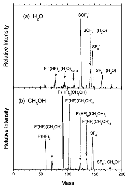
Figure 4. Mass spectra for reactions of \text{SF}_6^- with (a) \text{H}_2\text{O} and (b) \text{CH}_3\text{OH} at 100 Torr.
