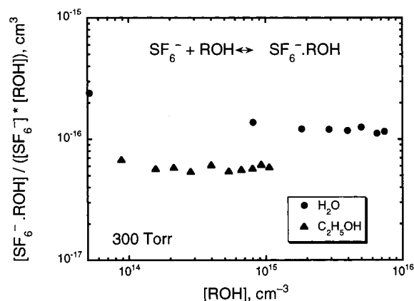
Figure 1. Demonstration of initial equilibrium for SF 6 - reacting with H 2 O and C 2 H 5 OH at 300 Torr. K' = [SF 6 - (ROH)]/[SF 6 - ][ROH].
