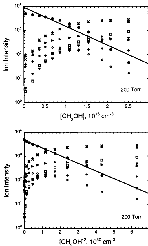
Figure 2. Example of data for reaction of SF 6 - with CH 3 OH at 200 Torr plotted as (a, top panel) pseudo-first-order kinetics and (b, bottom panel) pseudo-second-order kinetics. The species are represented as follows: (●) SF 6 - ; (○) SF 6 - (CH 3 OH); (arrowhead pointing right) F - (HF) 2 ; (△) F - (HF) 2 (CH 3 OH); (▽) F - (HF) 2 (CH 3 OH) 2 ; (+) F - (HF)(CH 3 OH) 2 ; (×) F - (HF)(CH 3 OH) 2 ; (□) F - (HF)(CH 3 OH) 3 .
