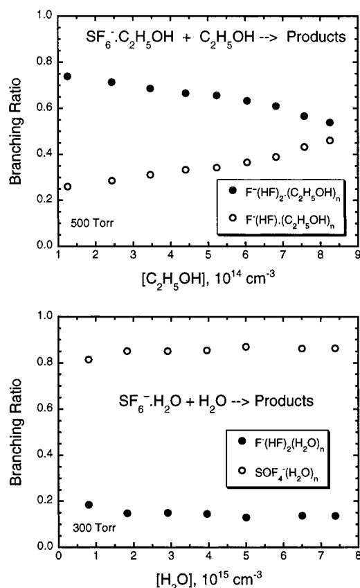
Figure 5. Product plot for (a, top panel) \text{C}_2\text{H}_5\text{OH} reaction at 500 Torr and (b, bottom panel) \text{H}_2\text{O} reaction at 300 Torr.
