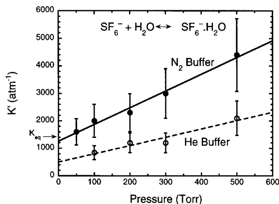
Figure 3. Pressure dependence of K' for \text{H}_2\text{O} reaction, shown for both \text{N}_2 and \text{He} buffers. Actual K_{\text{eq}} , as determined by Sieck, 4 is shown on y-axis.
