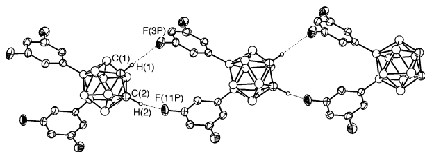
Fig. 2 Crystal packing diagram of 2 . The three molecules are related by translation. Selected distances (Å) and angles (°): C(1)⋯F(3P) 3.462(5), H(1)⋯F(3P) 2.47, C(2)⋯F(11P) 3.107(5), H(2)⋯F(11P) 2.35; C(1)–H(1)–F(3P) 160, C(2)–H(2)–F(11P) 124. For clarity, the remaining phenyl and carborane H atoms are not shown.
