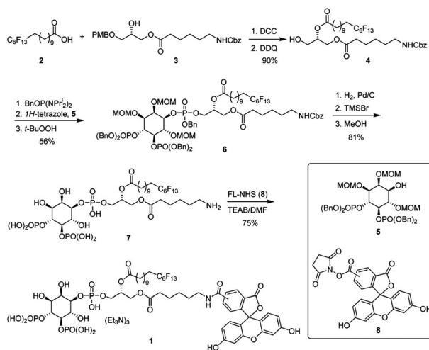
Scheme 1 Synthesis of the fluororous substrate PtdIns(4,5)P 2 .
