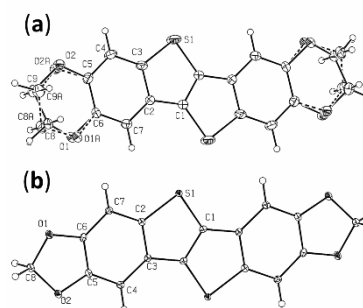
Figure 2. (a) and (b) : A molecular view of compounds 2 and 3 , respectively, showing the atom-labelling scheme. Displacement ellipsoids are drawn at 30% probability level. Unlabelled atoms are generated by symmetry. A detailed crystal data table is given in Table S1 as supporting information.
