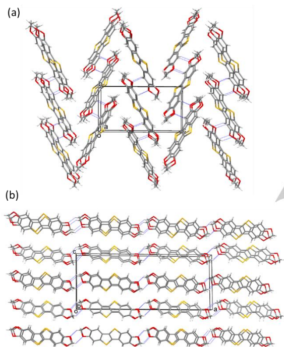
Figure 3. (a) Crystal packing diagram for compound 2 . C-H...O bonds are shown with dotted lines while the stacked molecules interact via \pi ... \pi interactions. (b) Crystal packing diagram for compound 3 . C-H...O bonds are shown with dotted lines while the stacked molecules interact via \pi ... \pi interactions leading to a parallel two dimensional network in the crystallographic b-direction.
