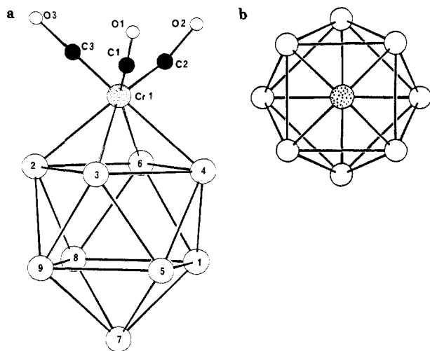
Figure 1. Chem-X 24 ball-and-stick representations of the \text{Sn}_9\text{Cr}(\text{CO})_3^{4-} ion as viewed (a) side-on and (b) down the Cr-Sn(7) vector showing the highly regular cluster geometry (carbonyl ligands omitted for clarity). Pertinent distances (Å) and angles (deg) [averaged where appropriate]: Cr(1)-Sn(3) = 2.890 (6), Cr(1)-Sn(6) = 2.859 (6), Cr(1)-Sn(2) = 2.867 (6), Cr(1)-Sn(4) = 2.869 (6), Cr(1)-C(1) = 1.71 (3), Cr(1)-C(2) = 1.66 (4), Cr(1)-C(3) = 1.71 (4), C(1)-O(1) = 1.27 (4), C(2)-O(2) = 1.26 (4), C(3)-O(3) = 1.29 (5), Sn(7)-Sn(1,5,8,9) = 2.94 (2), Sn(3)-Sn(6) = 4.35 (2), Sn(2)-Sn(4) = 4.33 (2), Sn(8)-Sn(5) = 4.43 (2), Sn(9)-Sn(1) = 4.49 (2), Cr(1)-C(1)-O(1) = 173 (3), Cr(1)-C(2)-O(2) = 170 (3), Cr(1)-C(3)-O(3) = 176 (3).
