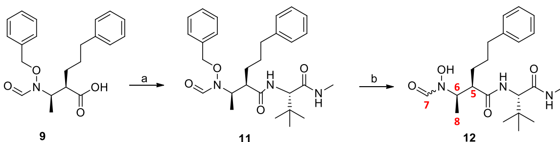
Scheme 7. Reagents and Conditions: (a) 10 , DCC, HOBT, DMAP, 0 °C – rt, 65%; (b) Pd/C, H 2 , rt, 97%.
