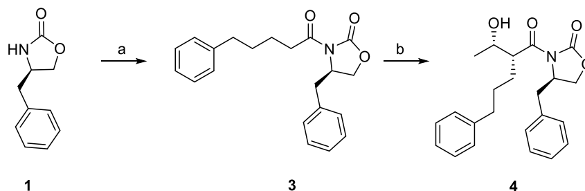
Scheme 3. Reagents and conditions: a) (i) n -BuLi, THF, -78 - 0\text{ }^{\circ}\text{C} , (ii) 5-Phenylpentanoyl chloride ( 2 ), 70%; b) (i) \text{Bu}_2\text{BOTf} , \text{Et}_3\text{N} , DCM, 0\text{ }^{\circ}\text{C} , (ii) \text{CH}_3\text{CHO} , -78\text{ }^{\circ}\text{C} , 90%.
