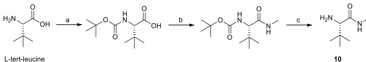
Scheme 6. Reagents and conditions: (a) \text{Boc}_2\text{O} , KOH, THF:H 2 O, rt, 87%; (b) EDC.HCl, HOBT, Et 3 N, H 2 CNH 2 .HCl, DCM 0 °C – rt, 90%; (c) TFA, DCM, 0 °C, 86%.
