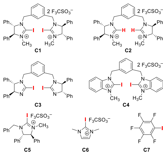
Figure 1. Halogen-bond donors C1 – C7 .
