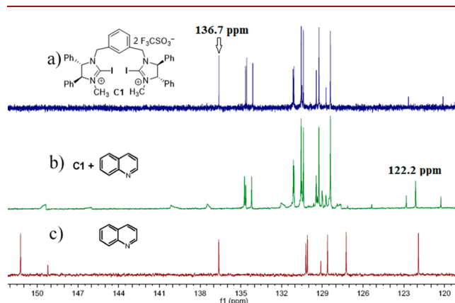
Figure 3. 13 C NMR spectra of C1 and 1a in CD 2 Cl 2 : (a) C1 ; (b) C1 + 1a (1:1); (c) 1a .
