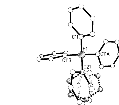
Figure 1. A ball-and-stick diagram of the disordered \text{Ph}_4\text{P}^+ in 1.
