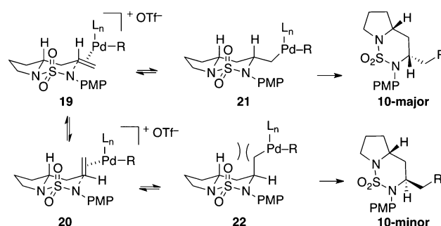
Scheme 3. Stereochemical Model
