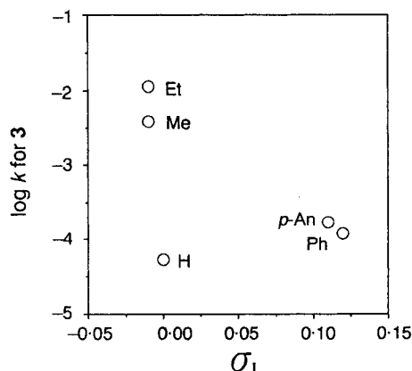
Figure 1. Plot of log k for 3 in 80% EtOH at 25 °C against \sigma_I
