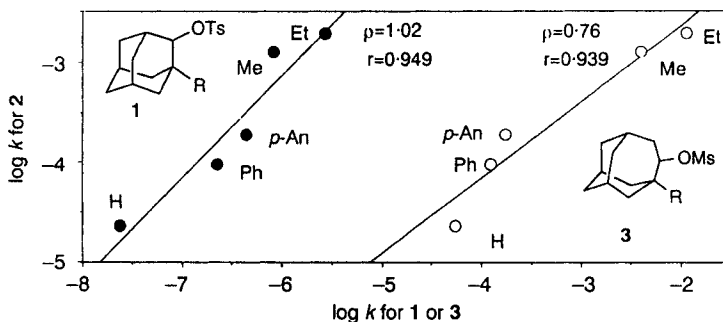
Figure 2. Plot of log k for 2 in AcOH against log k for 1 and 3 in 80% EtOH at 25 °C. (•) 1 vs 2 ; (○) 3 vs 2
