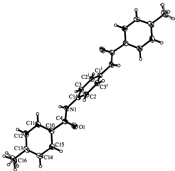
Fig. 1. View of the anisotropic displacement ellipsoids (50% probability) for the C, N and O atoms of (I) and the numbering scheme.
