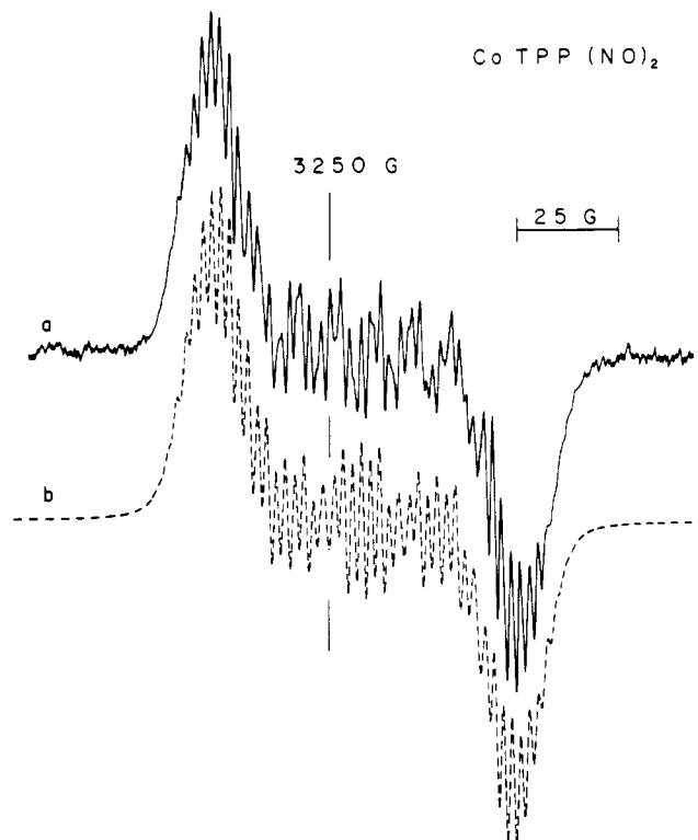
Figure 7. EPR spectrum for CoTPP(NO) 2 in toluene solution (230 K): (a) (—) observed spectrum; (b) (---) computer simulation using \langle g \rangle = 2.007 , \langle A(^{59}\text{Co}) \rangle = 9.3 G, \langle A(^{14}\text{N}(\text{NO})) \rangle = 4.15 G, and \langle A(^{14}\text{N}(\text{por})) \rangle = 2.3 G.
