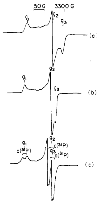
Figure 2. EPR spectra in frozen toluene media (100 K) for (a) \text{RhOEP}(\text{O}_2) , (b) \text{RhOEP}(\text{O}_2)(\text{pip}) , and (c) \text{RhOEP}(\text{O}_2)(\text{P}(\text{OBu})_3) .
