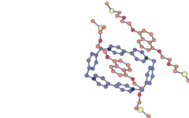
Figure 9. Geometry adopted by the complex formed between the \pi electron rich compound 17 and the tetracationic cyclophane 27 ·4PF 6 in the solid state.
