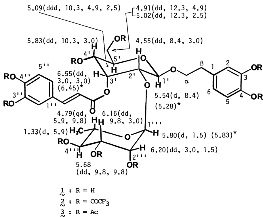
Fig. 1. Magnoloside A pertrifluoroacetate ( \sim 2 ): Pertinent ^1\text{H} NMR (400 MHz, pyridine- \text{d}_5 ) signals are shown; * are chemical shifts in magnoloside A ( \sim 1 ).
