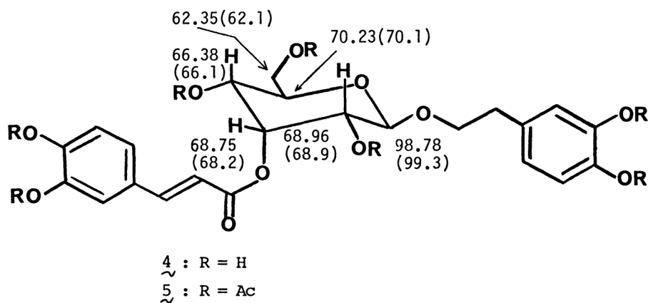
Fig. 2. ^{13}\text{C} NMR data (62.9 MHz, \text{CDCl}_3 ) for \sim 5 . Chemical shifts of methyl-2,3,4,6-tetraacetyl- \beta -D-allopyranose are given in parentheses.
