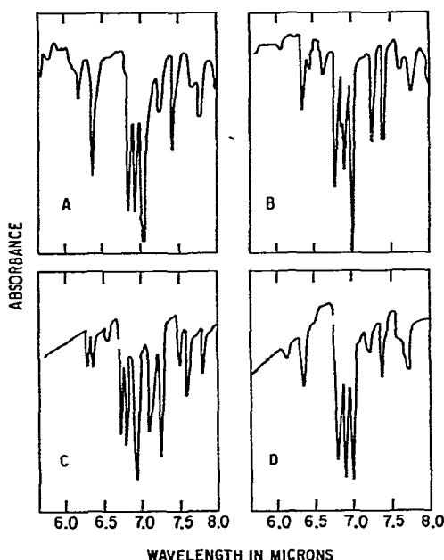
Fig. 1. Infrared spectra of (2- cis -propenylphenyl)diphenylphosphine ( cis -PP) and its complexes: A. cis -PP in deuteriochloroform solution 1a ; B. ( cis -PP)Cr(CO) 4 in deuteriochloroform 1a ; C. ( cis -PP)V(CO) 4 in Nujol (ca. 5.5–6.7 μm) and in hexachlorobutadiene (6.7–8.0 μm) mulls; D. [( cis -PP) uo V(CO) 5 ] − as the NPr 4 + salt in Nujol (ca. 5.5–6.7 μm) and in hexachlorobutadiene (6.8–8.0 μm) mulls.
