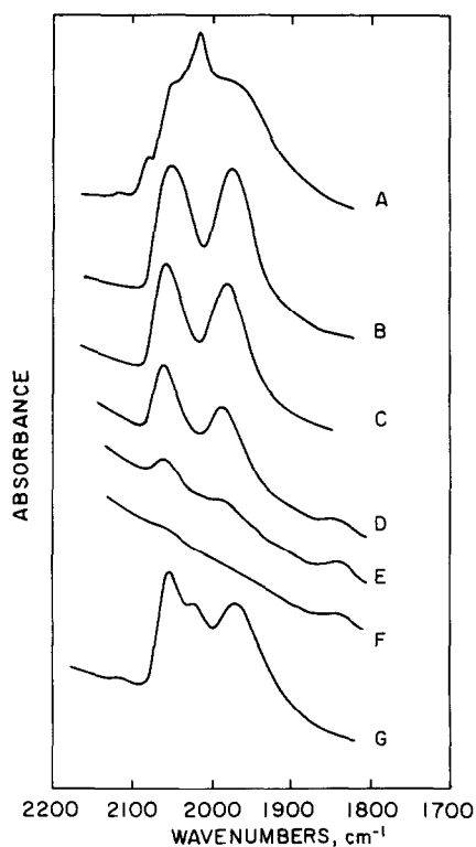
Fig. 7. IR spectra of sample prepared from [\text{H}_4\text{Ru}_4(\text{CO})_{12}] and \text{MgO} after treatment in air at various temperatures. A, initial sample; B, 58 °C, 30 min; C, 77 °C, 30 min; D, 100 °C, 30 min; E, 123 °C, 35 min; F, 149 °C, 30 min; G, F, followed by exposure to \text{CO} at 101 °C for 30 min.
