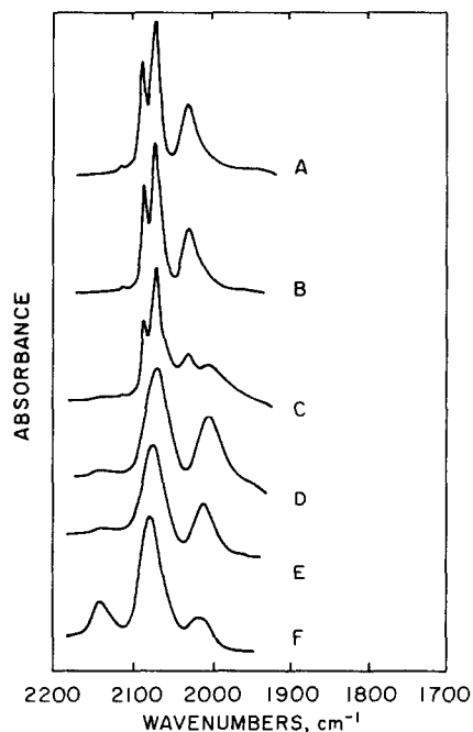
Fig. 1. IR spectra of sample prepared from [\text{H}_4\text{Ru}_4(\text{CO})_{12}] and \text{SiO}_2 after treatment in air at various temperatures. A, initial sample; B, 51^\circ\text{C} , 30 min; C, 75^\circ\text{C} , 20 min; D, 98^\circ\text{C} , 20 min; E, 122^\circ\text{C} , 20 min; F, 150^\circ\text{C} , 2 h, followed by exposure to CO at 95^\circ\text{C} for 1 h (spectra were corrected by subtraction of absorption by the \text{SiO}_2 support).
