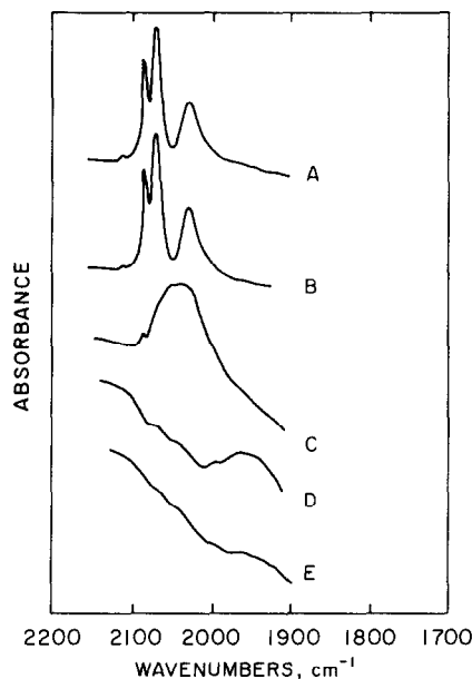
Fig. 2. IR spectra of sample prepared from [\text{H}_4\text{Ru}_4(\text{CO})_{12}] and \text{SiO}_2 after treatment in hydrogen at various temperatures. A, initial sample; B, 53^\circ\text{C} , 30 min; C, 75^\circ\text{C} , 30 min; D, 100^\circ\text{C} , 30 min; E, 350^\circ\text{C} , 30 min, followed by exposure to CO at 98^\circ\text{C} for 1 h (spectra were corrected by subtraction of absorption by the \text{SiO}_2 support).
