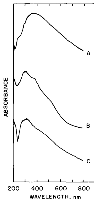
Fig. 3. UV–Vis spectra of supported ruthenium samples after treatment in helium at 150 °C. A, sample prepared from [H_4Ru_4(CO)_{12}] and SiO 2 ; B, sample prepared from [H_4Ru_4(CO)_{12}] and \gamma -Al 2 O 3 ; C, sample prepared from [H_4Ru_4(CO)_{12}] and MgO.
