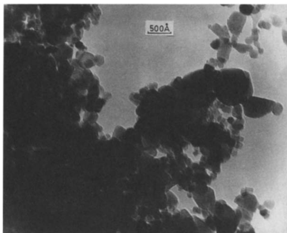
Fig. 6. Electron micrograph showing ruthenium metal particles formed by reduction (at 350 °C in hydrogen) of sample prepared from [\text{H}_4\text{Ru}_4(\text{CO})_{12}] and \text{TiO}_2 .
