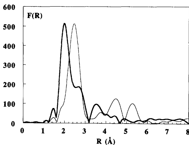
Fig. 4. Fourier transformed EXAFS spectrum (FT) of 1 (—) and Ti metal (—), phase shift not corrected. The intensity of the FT for 1 is in fact approximately 1/3 of that for Ti metal and was normalized here to aid in the visual comparison.
