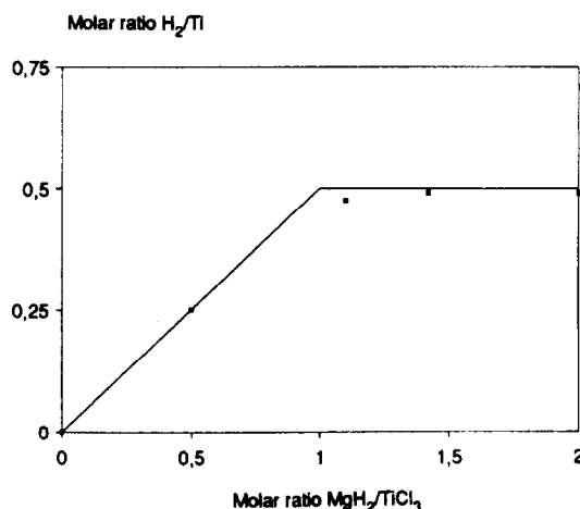
Fig. 1. Hydrogen evolution as a function of the molar ratio of the reactants in the reduction of [TiCl 3 (THF) 3 ] with MgH 2 ' in THF (0–25°C).
