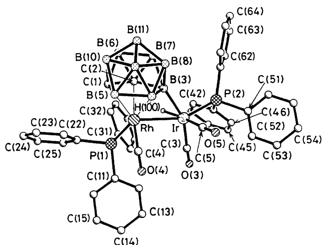
Figure 3. The molecular structure of the complex [\text{RhIrH}(\mu\text{-}\sigma\text{:}\eta^5\text{-C}_2\text{B}_9\text{H}_{10})(\text{CO})_3(\text{PPh}_3)_2] (4) showing the crystallographic numbering scheme
