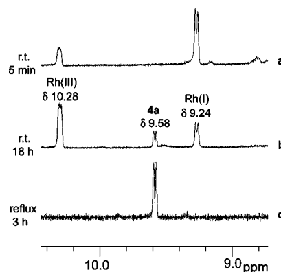
Figure 4. H6 of the pyridine ring monitored by ^1\text{H} NMR spectroscopy.
