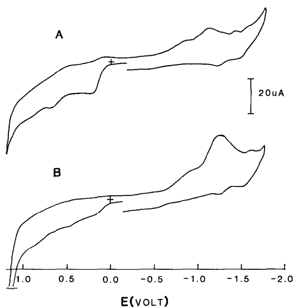
Fig. 7. Cyclic voltammograms of 1.0 mM \text{VO}(\text{Pen-OCH}_3)_2 + 0.1 \text{ mM } [(\text{bpy})_2\text{Ru}(\text{tri-n-Bu})\text{P}]\text{Cl})\text{PF}_6 in 0.1 M TEAP/DMSO, at a platinum electrode. Scan rate 200 mV/s. A, Original solution; B, after complete oxidation at 0.6 V.
