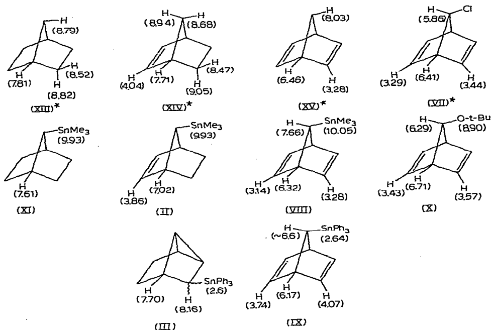
Fig. 1. Proton chemical shifts of some norbornane derivatives and their organotin analogues ( \tau values in parentheses).
