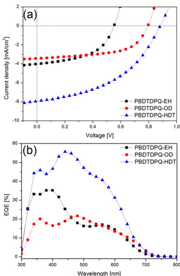
FIGURE 4 (a) The J–V characteristics and (b) IPCE spectra of BHJ solar cells with the device. [Color figure can be viewed in the online issue, which is available at wileyonlinelibrary.com .]
