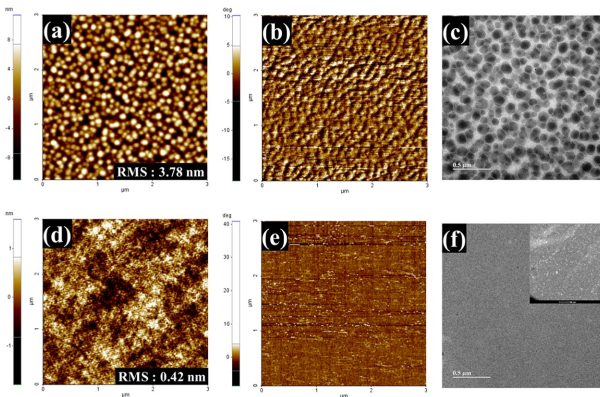
FIGURE 5 Topographic AFM images (a, d), phase images (b, e), and TEM images (c, f) of PBDDTPQ-OD:PC 71 BM (1:1 wt/wt, 3 \times 3 \mu\text{m}^2 ) (a–c) and PBDDTPQ-HDT:PC 71 BM (1:3 wt/wt, 3 \times 3 \mu\text{m}^2 ) (d–f), (inset of (f): STEM image). [Color figure can be viewed in the online issue, which is available at wileyonlinelibrary.com .]
