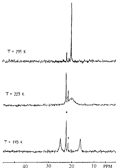
Fig. 3. Variable ^{31}\text{P} NMR spectra (81 015 MHz, \text{CD}_2\text{Cl}_2 ) for complex 5 , * due to traces of complex 3 and + of dpnapy oxide
