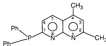
Fig. 1 7-Diphenylphosphino-2,4-dimethyl-1,8-naphthyridine
