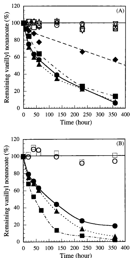
Figure 2. Change in vanillyl nonanoate with time in various solvents (A) and several solvents containing water (B) at 25 °C: (A) (□) nonsolvent, (○) ethyl acetate, (◇) chloroform, (Δ) hexane, (▽) acetone, (◆) dimethyl sulfoxide, (●) methanol, (▲) ethanol, and (■) aqueous surfactant vehicle (0.9% NaCl aqueous solution containing 2% ethanol and 10% Tween 80); (B) (□) ethyl acetate with 1% water, (○) water-saturated ethyl acetate, (●) methanol with 1% water, (▲) ethanol with 1% water, and (■) methanol with 50% water.
