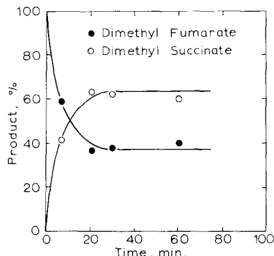
Fig. 2. Dimethyl fumarate and \text{HCo}(\text{CO})_4 (1/1). Dimethyl fumarate, 2.26 mmoles; \text{HCo}(\text{CO})_4 , 2.27 mmoles; toluene solvent 15 ml; temp. 26^\circ ; CO atm.; quenched with triphenylphosphine to remove cobalt complexes before analysis.
