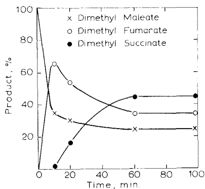
Fig. 1. Dimethyl maleate and \text{HCo}(\text{CO})_4 (1/1). Dimethyl maleate, 2.25 mmoles; \text{HCo}(\text{CO})_4 , 2.27 mmoles; toluene solvent is 15 ml; temp. 26^\circ ; CO atm.; quenched with triphenylphosphine to remove cobalt complexes before analysis.
