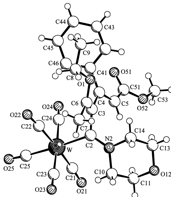
Fig. 2. Molecular structure of carbiminium carbonyltungstate 6a . Selected bond lengths (Å) and angles ( ^\circ ): W–C2 2.247(9), C2–N2 1.318(13), C2–C3 1.514(15), N2–C10 1.479(14), N2–C14 1.480(14), C11–C10 1.49(2), C3–C6 1.331(14), C3–C4 1.464(14), C6–O1 1.379(12), C6–C7 1.51(2), O1–C8 1.413(14), C8–C9 1.46(2), C4–C5 1.38(2), C4–C41 1.48(2), C5–C51 1.44(2), C51–O51 1.256(14), C51–O52 1.288(14), O52–C53 1.41(2); N2–C2–C3 114.4(9), N2–C2–W 129.8(8), C3–C2–W 115.7(6), C2–N2–C10 124.6(9), C2–N2–C14 125.2(10), C10–N2–C14 110.3(9), N2–C14–C13 109.9(11), N2–C10–C11 109.1(10), C6–C3–C4 123.2(10), C6–C3–C2 119.4(9), C4–C3–C2 117.4(9), C3–C6–O1 118.8(9), C3–C6–C7 124.2(10), O1–C6–C7 116.7(10), C6–O1–C8 118.8(9), C5–C4–C3 115.8(10), C5–C4–C41 123.8(10), C3–C4–C41 120.5(9), C42–C41–C4 120.8(11), C46–C41–C4 120.3(9), C4–C5–C51 128.3(11), O51–C51–O52 121.7(11), O51–C51–C5 125.3(12), O52–C51–C5 113.0(11), C51–O52–C53 122.8(12).
