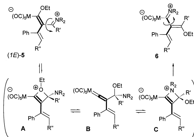
Scheme 3. Reaction path suggested for a 1,3 shift of the iminium functionality of carbiminium carbonylmetalates (1 E )- 5 .
