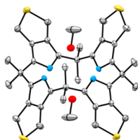
Figure 1. Single-crystal structure of 1 ·(CH 3 OH) 2 . Two molecules of methanol are H-bonded to two N–H's each. H-atoms were removed for clarity. Displacement ellipsoids are scaled to the 50% probability level.
