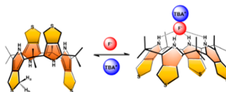
Figure 2. Schematic representation of electrostatic interactions that may stabilize the nonion paired complex obtained when receptor 1 is treated with TBAF in CDCl 3 .
