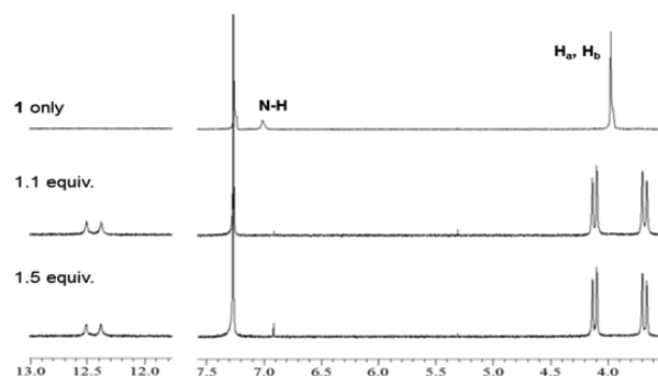
Figure 3. Partial 1 H NMR spectra recorded during the titration of receptor 1 (3.03 mM) with TEAF in CDCl 3 .
