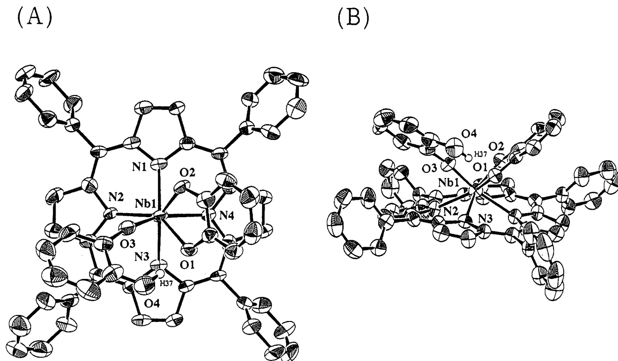
Figure 1. Molecular structure of Nb(tpp)(cat)(Hcat) (3): A, top view; B, side view. Coordinates of labeled atoms are given in Table 2.
