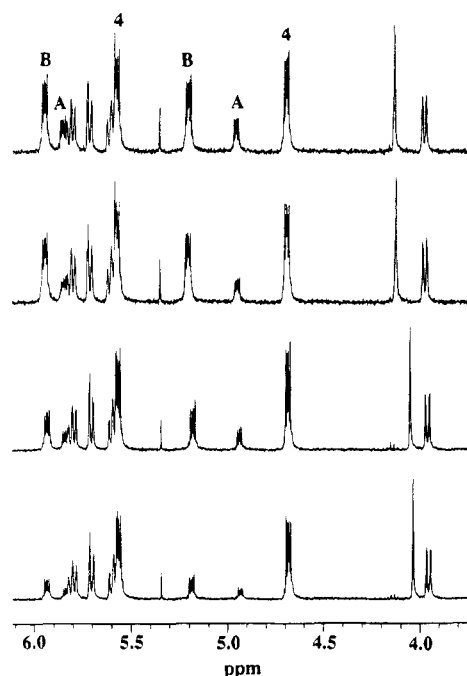
Figure 6. Time course of the ^1\text{H} -NMR spectrum of 2 in the region of catecholato ligands after addition of 2 equiv of catechol in \text{CDCl}_3 at -30^\circ\text{C} . Three labeled multiplet pairs correspond to intermediates A and B and the final complex 4 .
