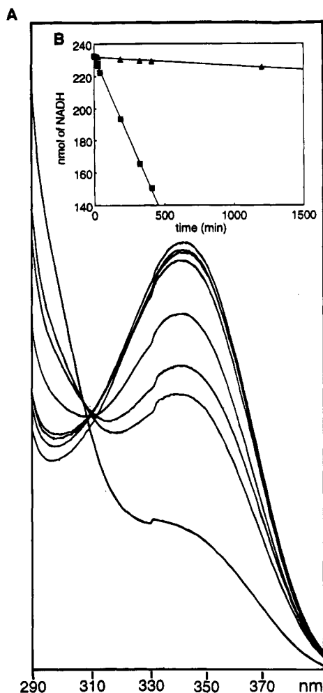
Figure 1. Incubation of myo -2-inositol 1-phosphate with the complex of NADH and apoMIP synthase: (A) The UV-vis absorbance profiles of the reaction solution at 0, 27, 27.5, 44, 186, 325, 408, and 1200 min when scanned from 250 to 400 nm; (B) the change in absorbance of the reaction solution when monitored at 340 nm with time (■); overlapping progress lines for control experiments where myo -2-inositol 1-phosphate was incubated with NADH in a solution lacking apoMIP synthase or in a separate experiment, where NADH was incubated with apoMIP synthase in a solution lacking myo -2-inositol 1-phosphate (▲).
