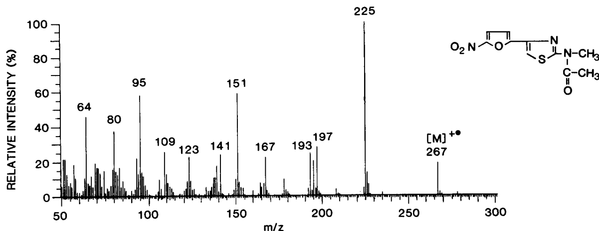
Figure 1. The low resolution mass spectrum of 2-acetyl-2-methylamino-4-(5-nitro-2-furyl)thiazole (Compound 2).
