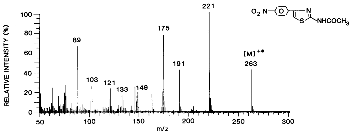
Figure 2. The low resolution mass spectrum of 2-acetyl-amino-4-(4-nitrophenyl)thiazole (Compound 3 ).
