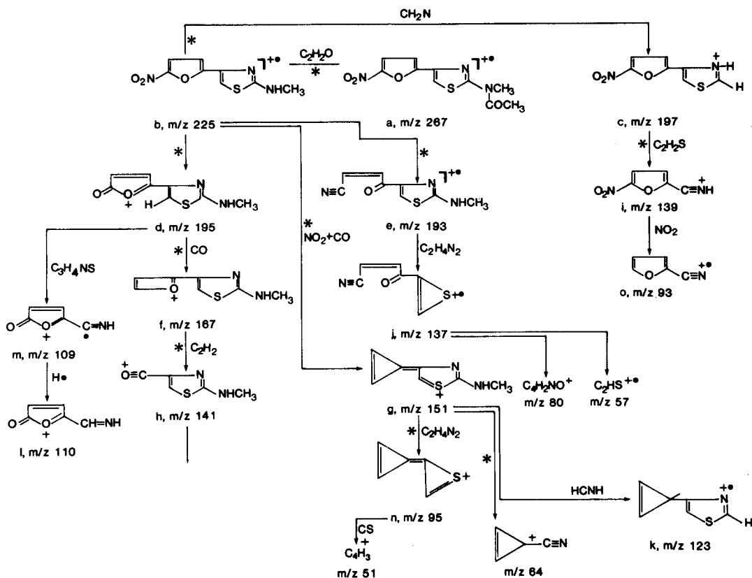
Scheme 1. Suggested fragmentation pathway of Compound 2.
