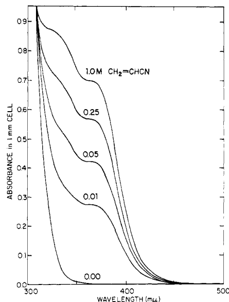
Figure 1. Optical spectra of benzene solutions at 40^\circ\text{C} containing 2.16 \times 10^{-3} \text{ M Ni[P(O-}i\text{-tolyl)}_3]_4 and increasing concentrations of acrylonitrile.
