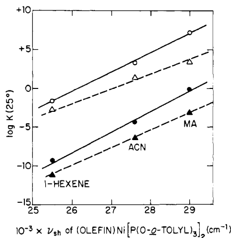
Figure 2. Plot of \log K (equilibrium constant) at 25 °C in benzene for the reaction \text{olefin} + \text{NiL}_4 = (\text{olefin})\text{NiL}_2 + 2\text{L} against \nu_{\text{sh}} for the (\text{olefin})\text{Ni}[\text{P}(\text{O-}o\text{-tolyl})_3]_2 complexes: \circ , \text{L} = \text{P}(\text{O-}o\text{-tolyl})_3 ; \Delta , \text{L} = \text{P}(\text{O-}i\text{-C}_6\text{H}_4\text{Cl})_3 ; \bullet , \text{L} = \text{P}(\text{O-}p\text{-tolyl})_3 ; \blacktriangle , \text{L} = \text{P}(\text{O-}p\text{-C}_6\text{H}_4\text{Cl})_3 .
